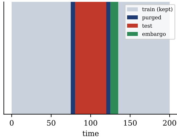
(b) purged k-fold anatomy, fold 3/5 ( h = 5 , embargo 5% of samples)
