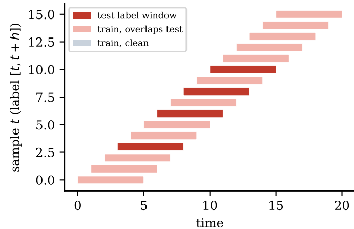
(a) shuffled k-fold, h = 5 : train windows overlap test windows
