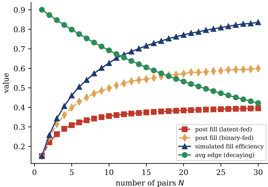
(a) fill efficiency vs avg edge
