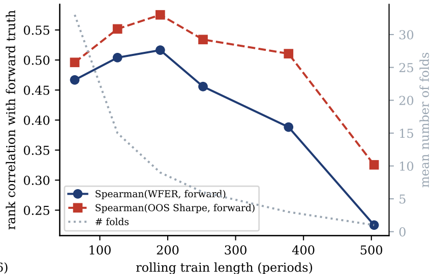
Diagnostic quality vs window length
