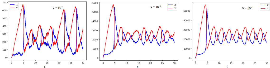
Figure 29: Oscillation in population during simulation time
