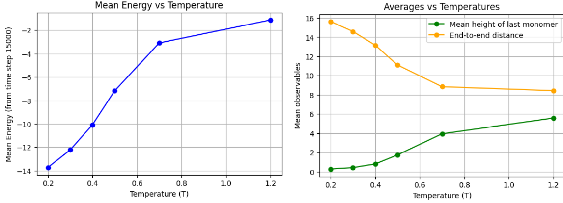
Figure 23: Left: mean energy per temperature. Right: mean end-to-end distance and mean height of the last monomer
