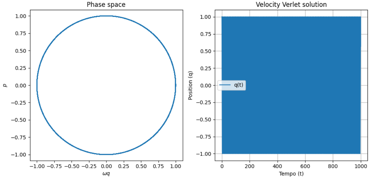
Figure 31: Phase space (left) and corresponding solution from Velocity Verlet algorithm (right), dt = 0.01 , \omega = 1
