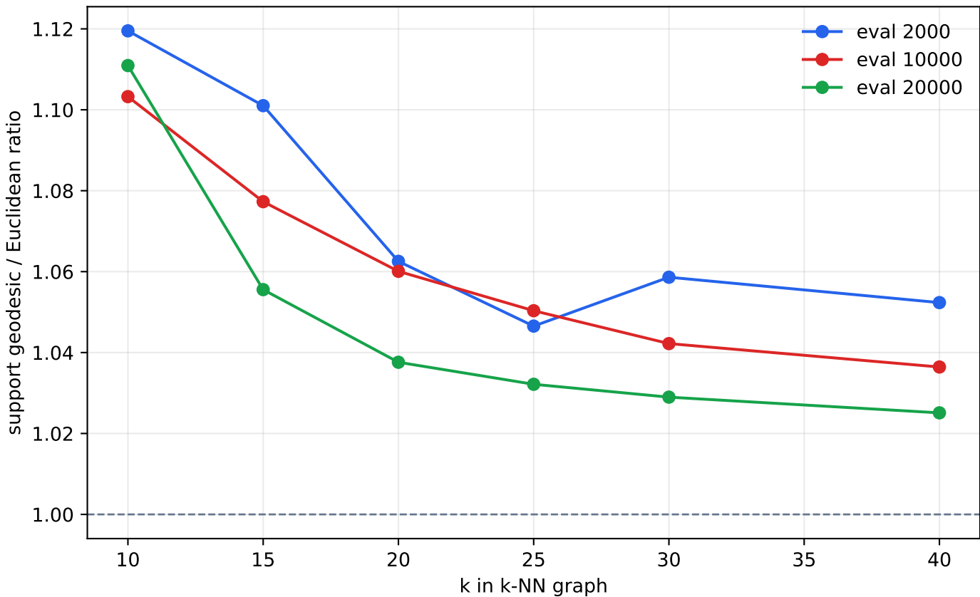
Dynamic Phase 4 graph k-sensitivity
