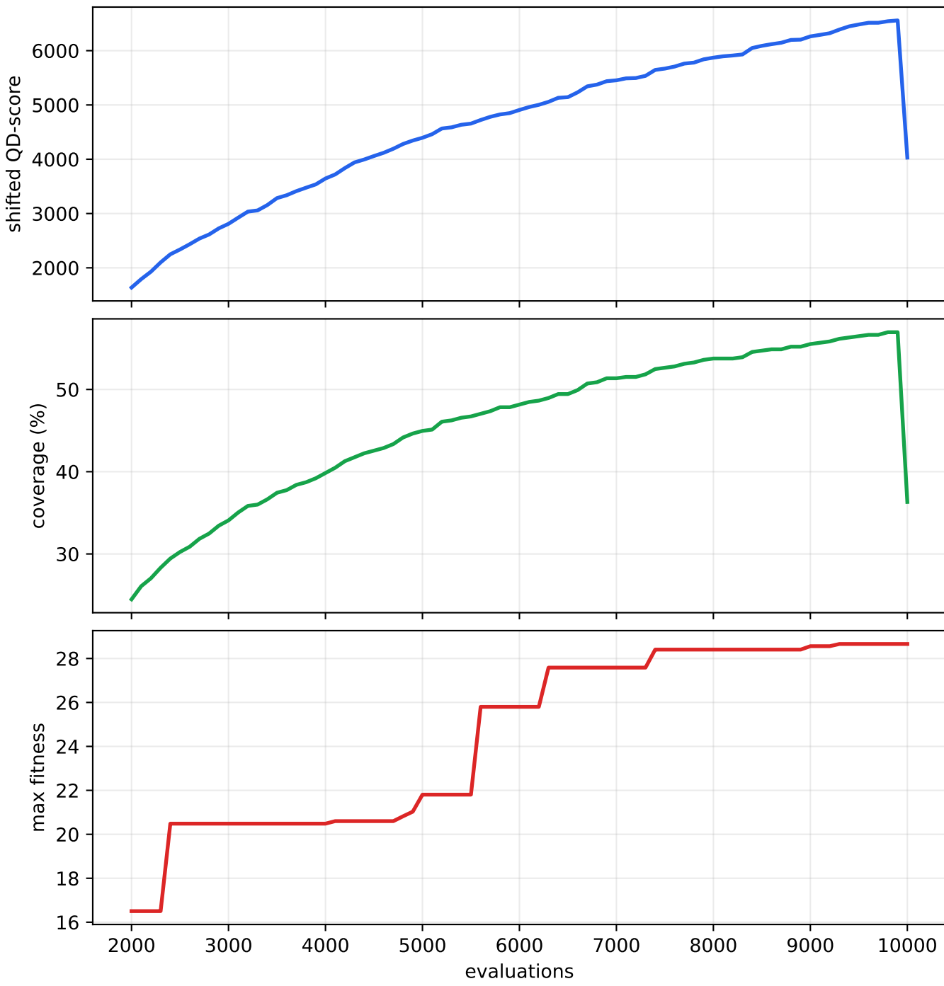
Normalization leakage audit only
