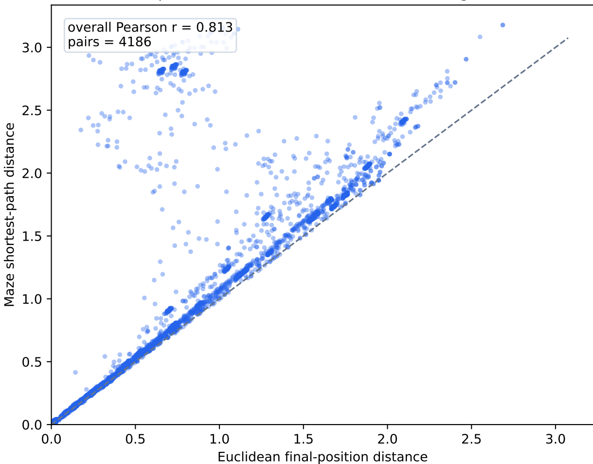
Final-position distances: Euclidean vs maze geodesic
