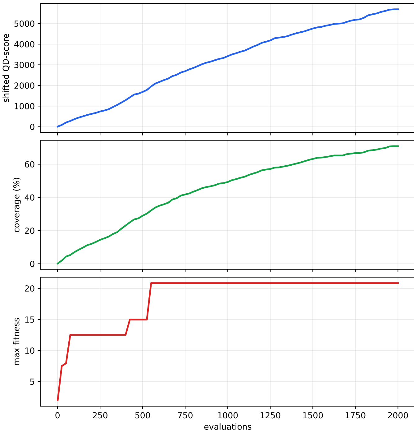
Phase 2 hand-crafted MAP-Elites progress
