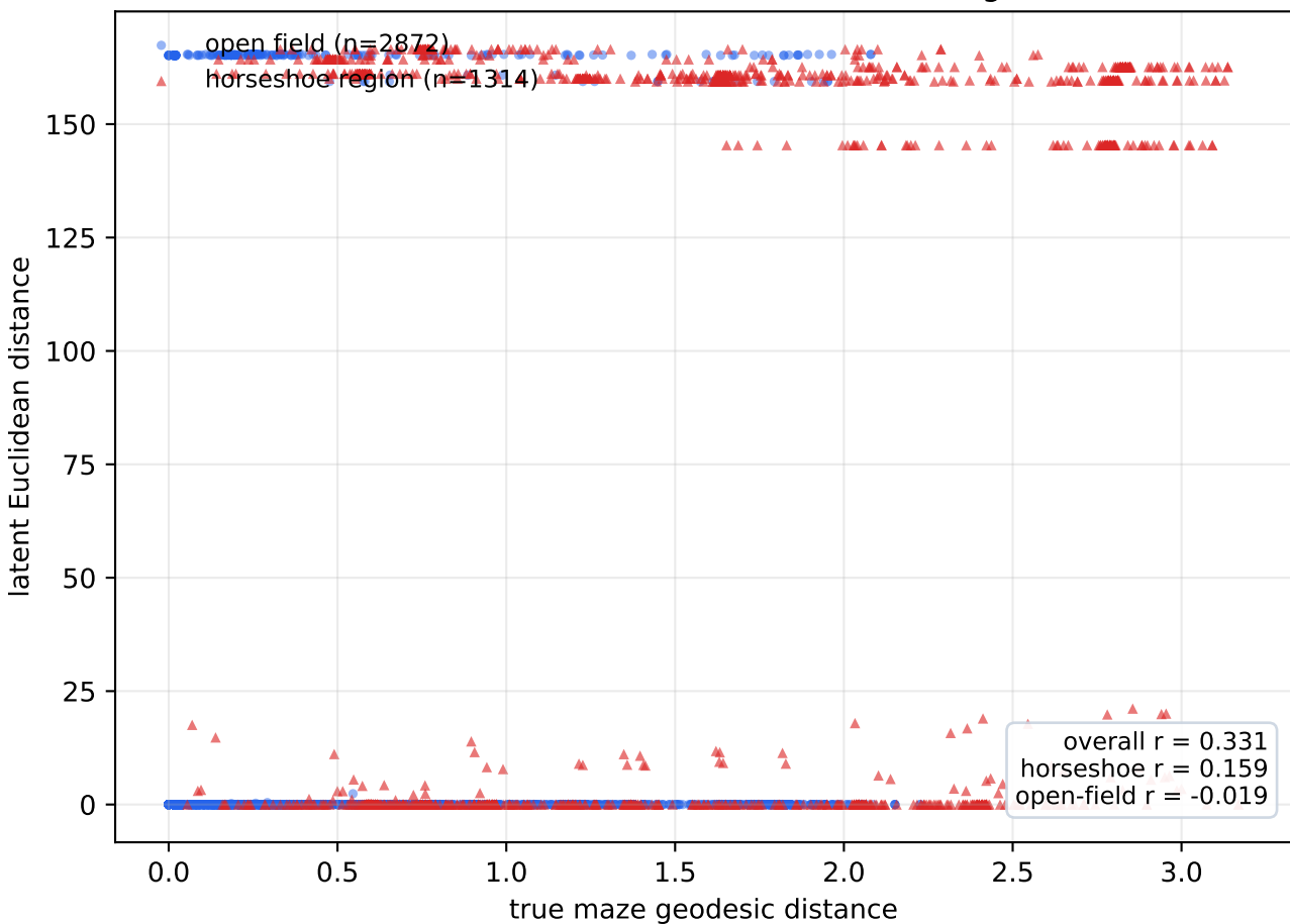
Locked Baseline B latent distance vs maze geodesic
