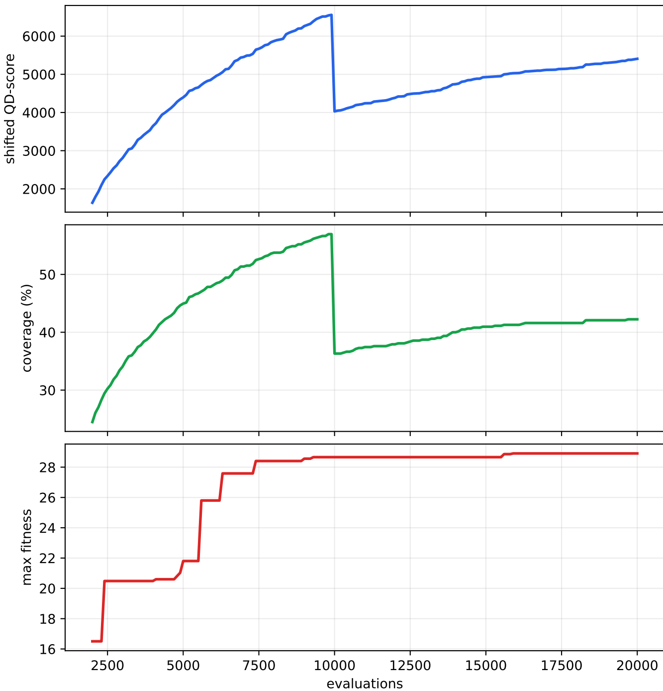
Phase 3 locked Baseline B one-retrain learned-BD baseline
