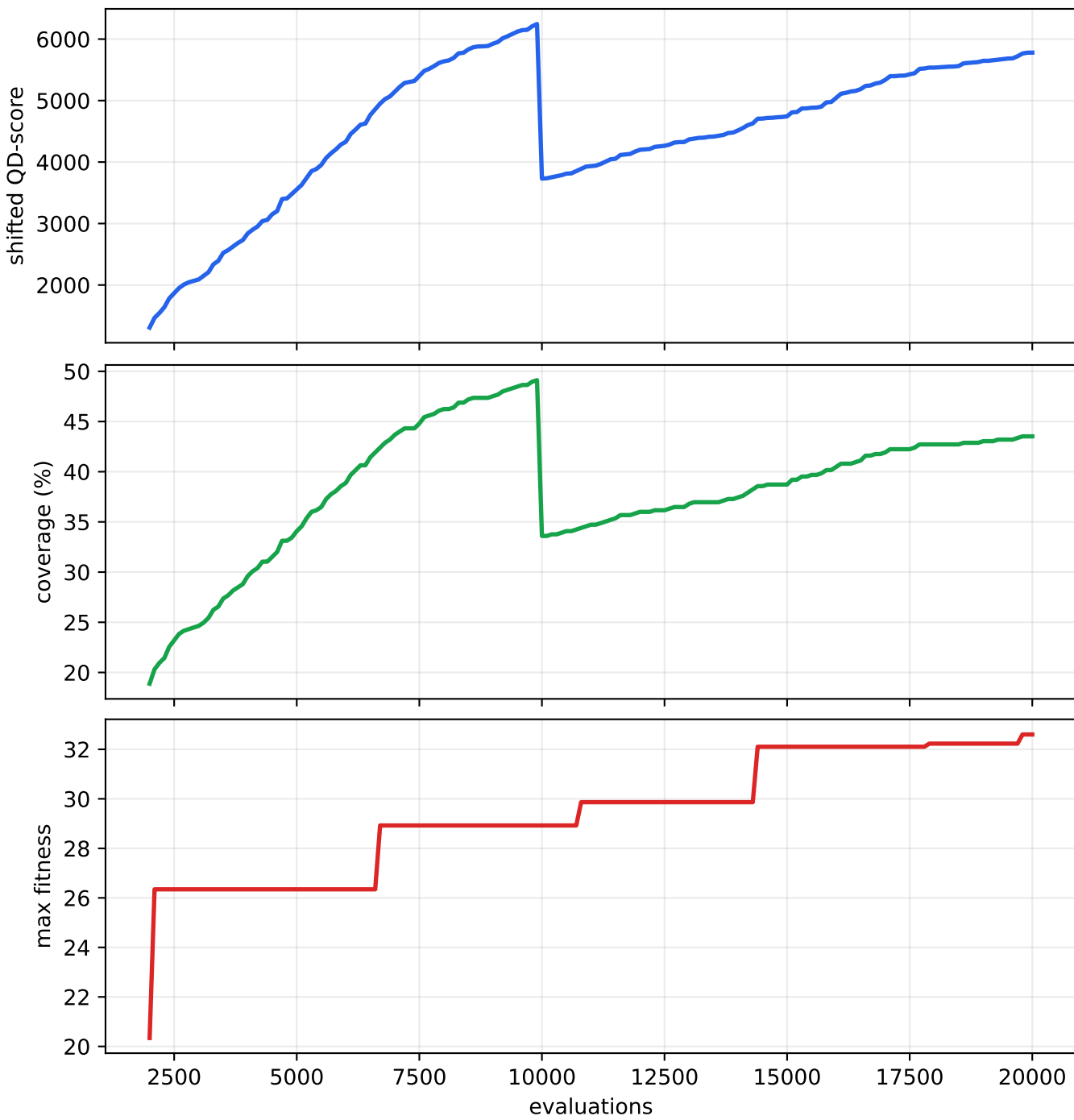
Phase 5 Baseline B: learned BD Euclidean seed 1002
