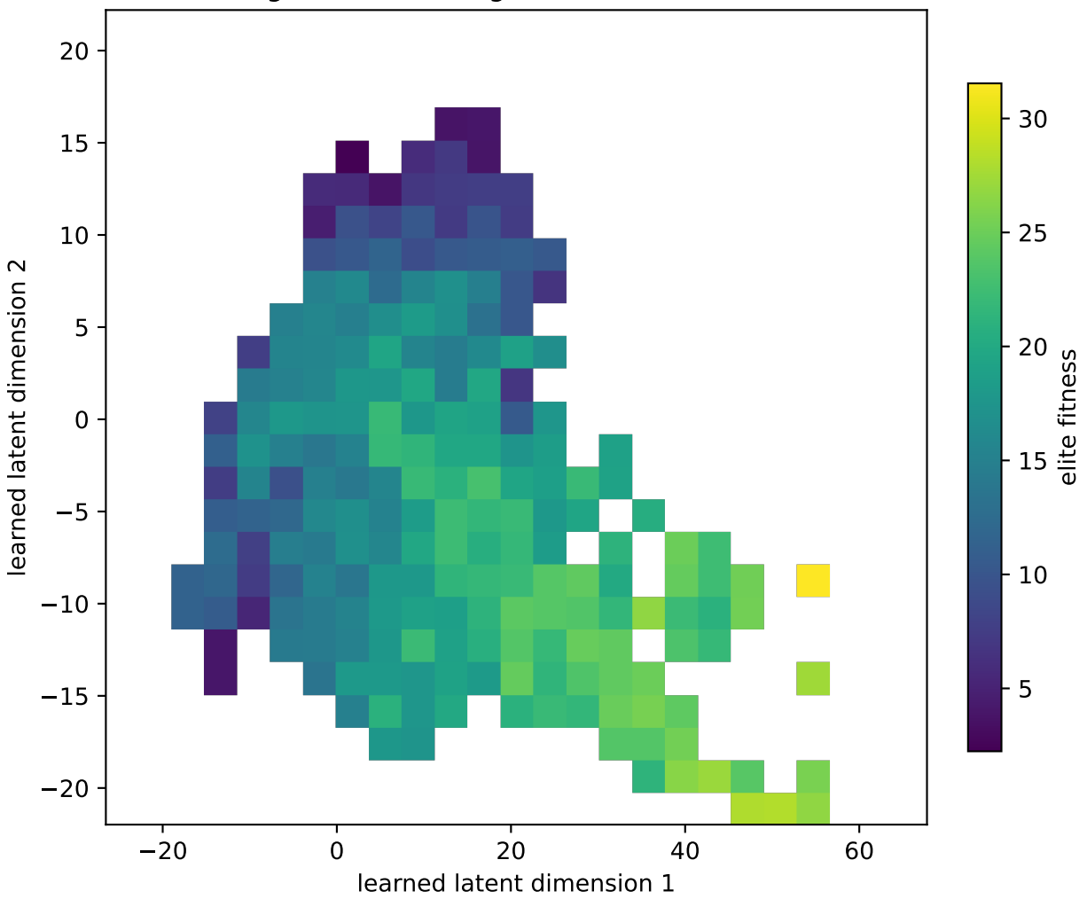
Phase 4 geodesic-niching archive: learned latent BD
