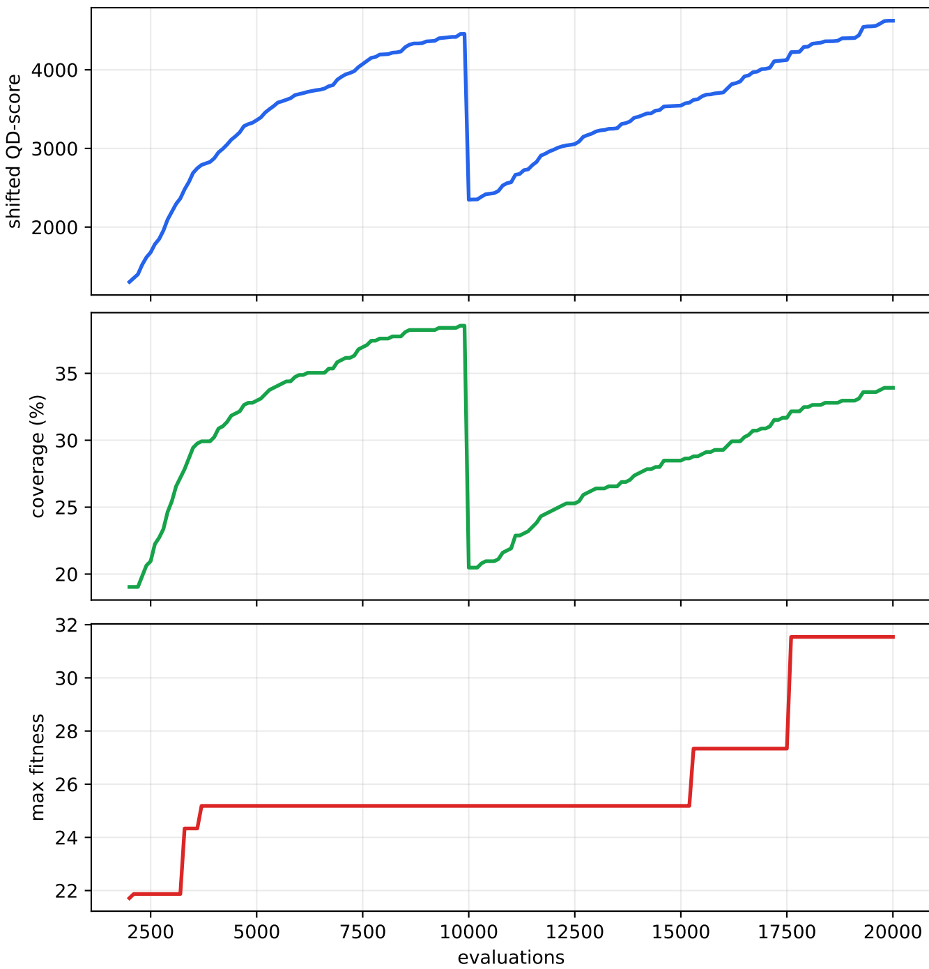
Phase 5 Contribution: geodesic niching seed 1003
