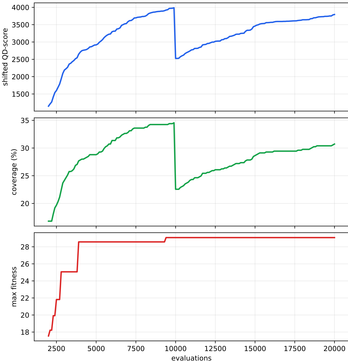
Phase 5 Contribution: geodesic niching seed 1005
