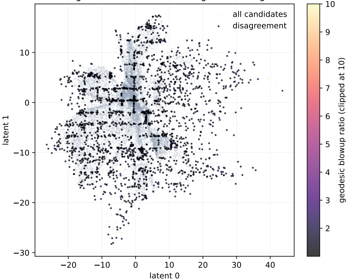
Seed 1005: geodesic vs Euclidean assignment disagreements
