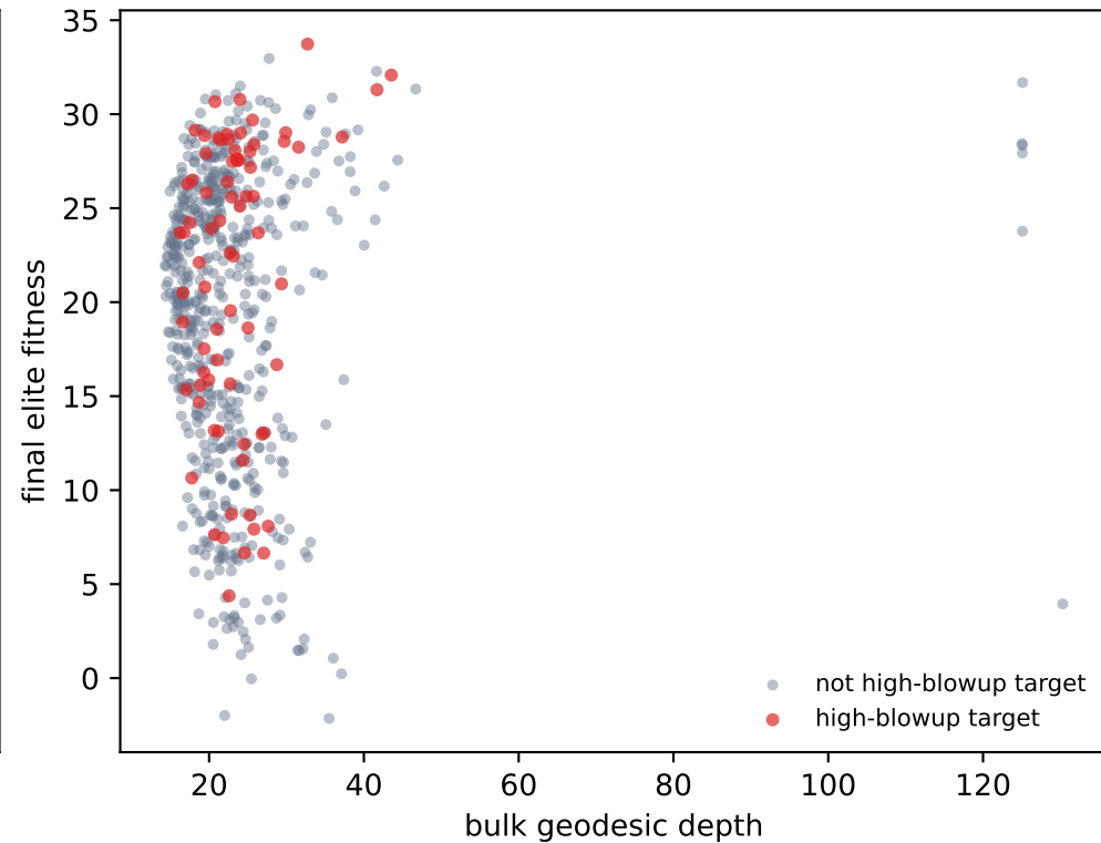
open robustness
