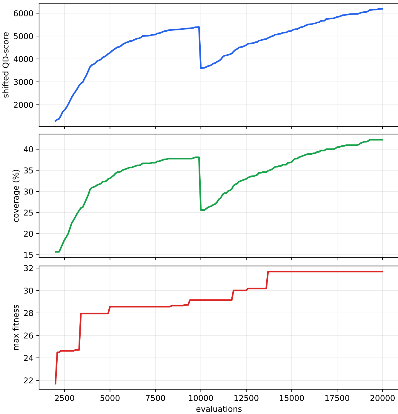
phase6_open_robustness Contribution: geodesic niching seed 1001
