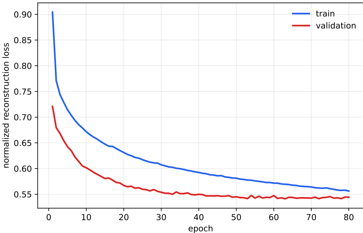
Phase 3 trajectory autoencoder loss
