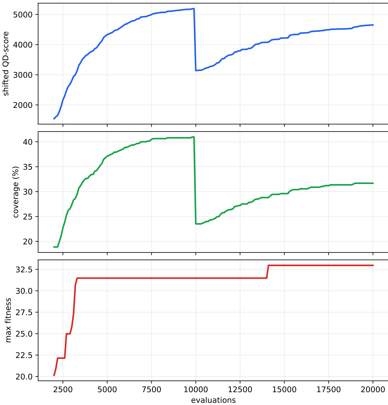
phase6_open_robustness Contribution: geodesic niching seed 1003
