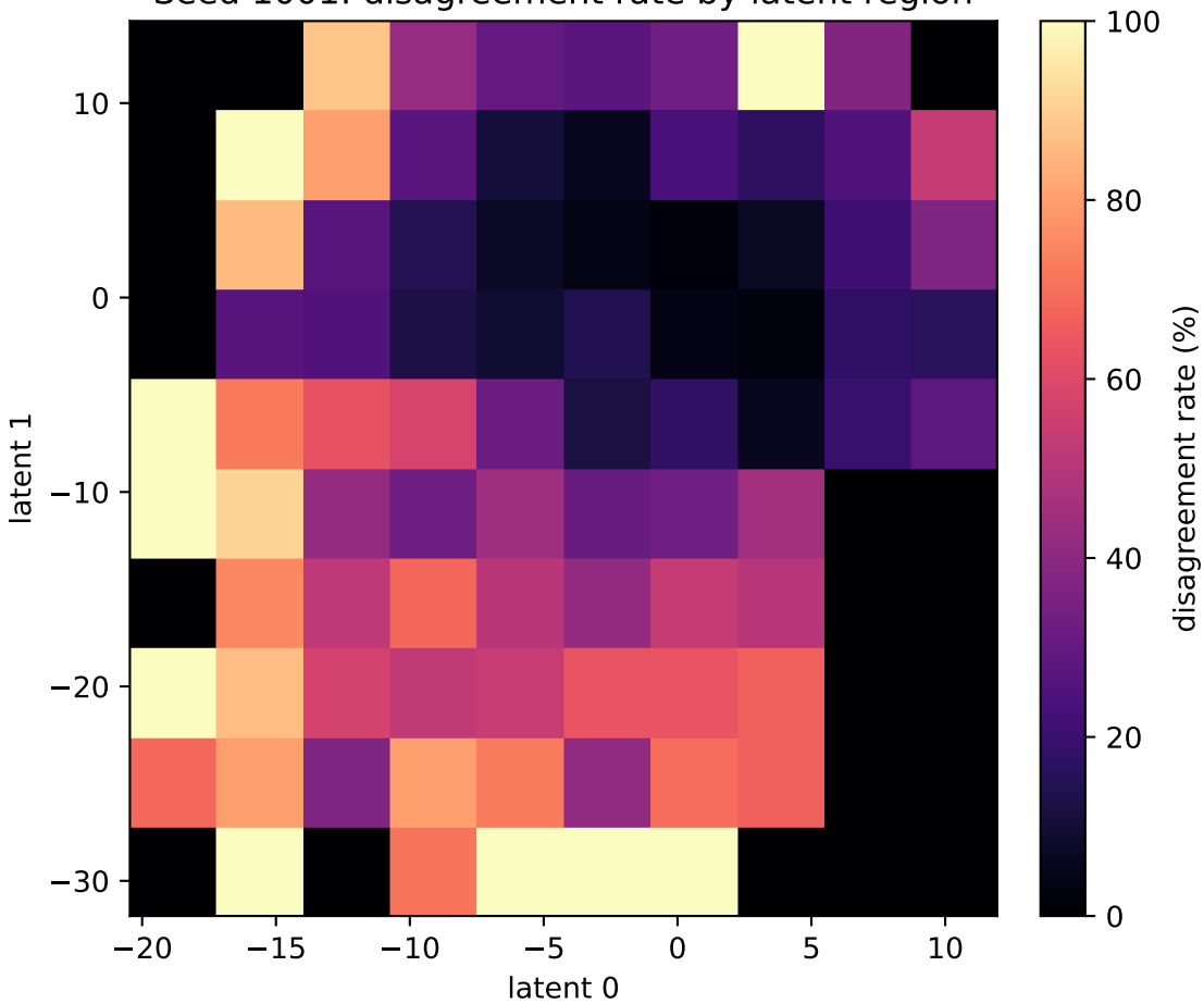
Seed 1001: disagreement rate by latent region
