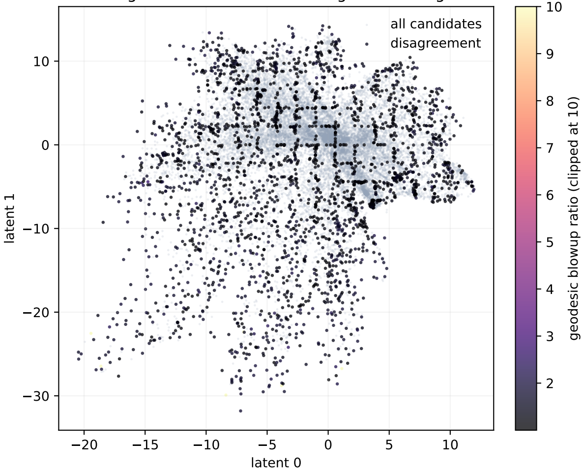
Seed 1001: geodesic vs Euclidean assignment disagreements
