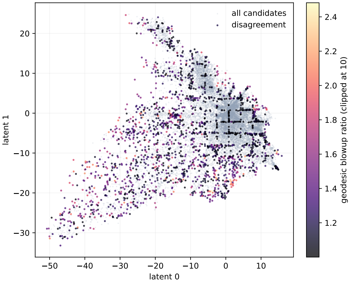
Seed 1002: geodesic vs Euclidean assignment disagreements
