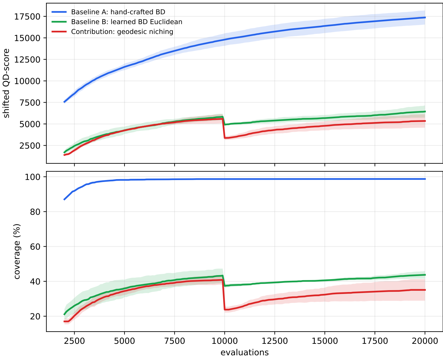
Phase 5 aggregate QD-score and coverage curves (mean \pm std)
