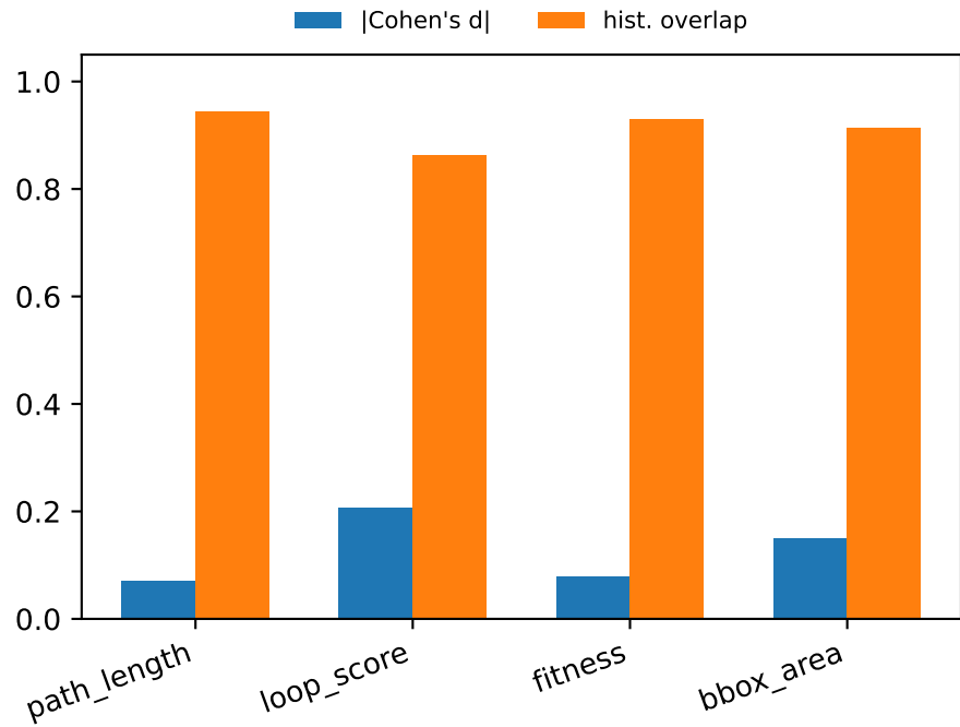
Distribution similarity
