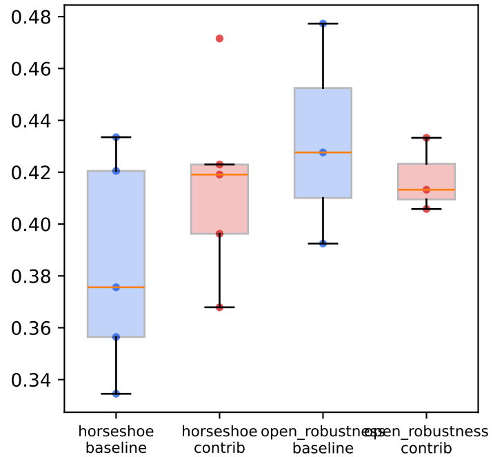
Mean pairwise distance
