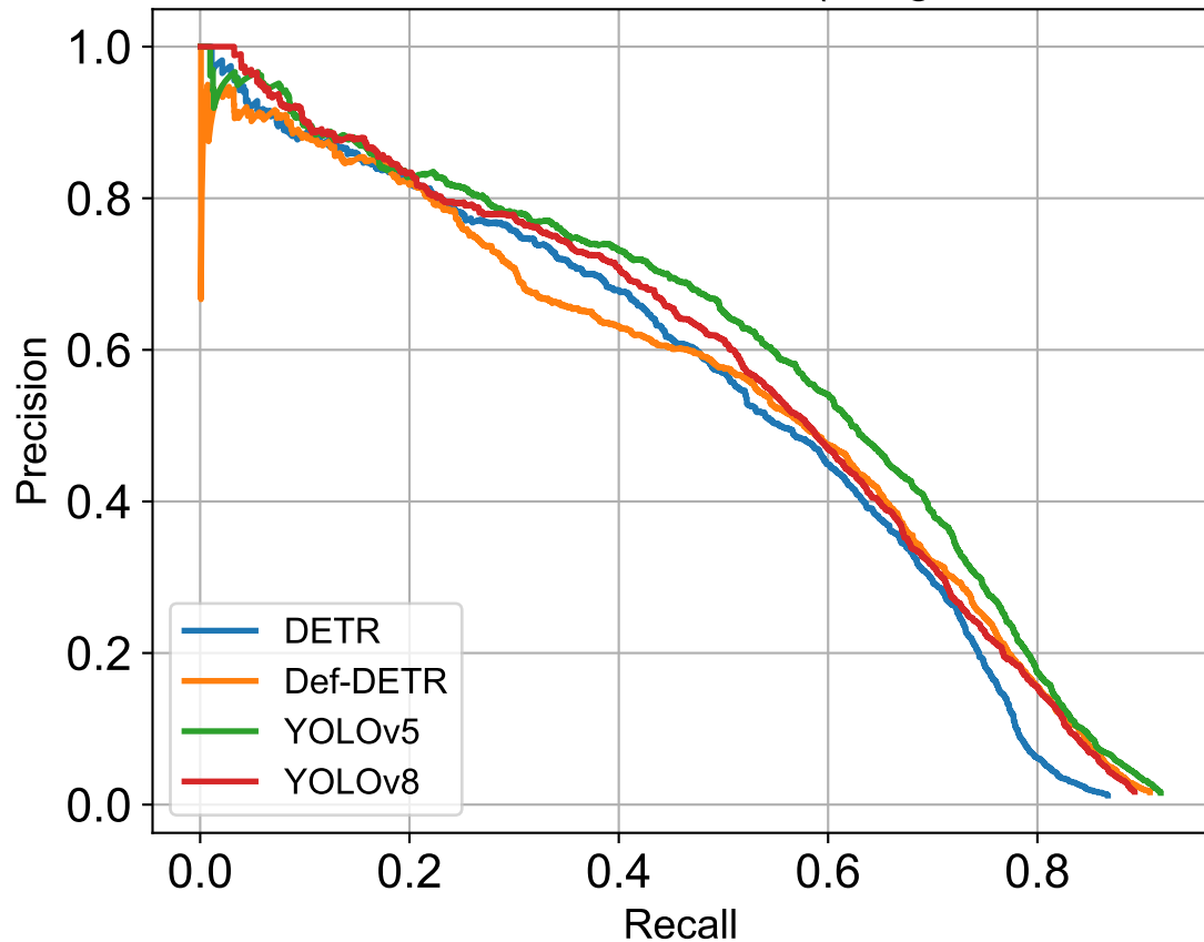
Precision-Recall Curves for D00 (Longitudinal Crack)
