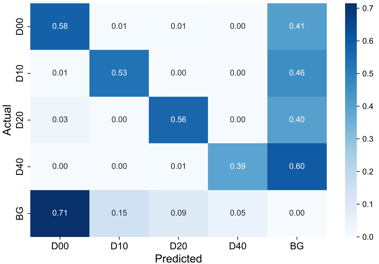
Confusion Matrix for YOLOv5
