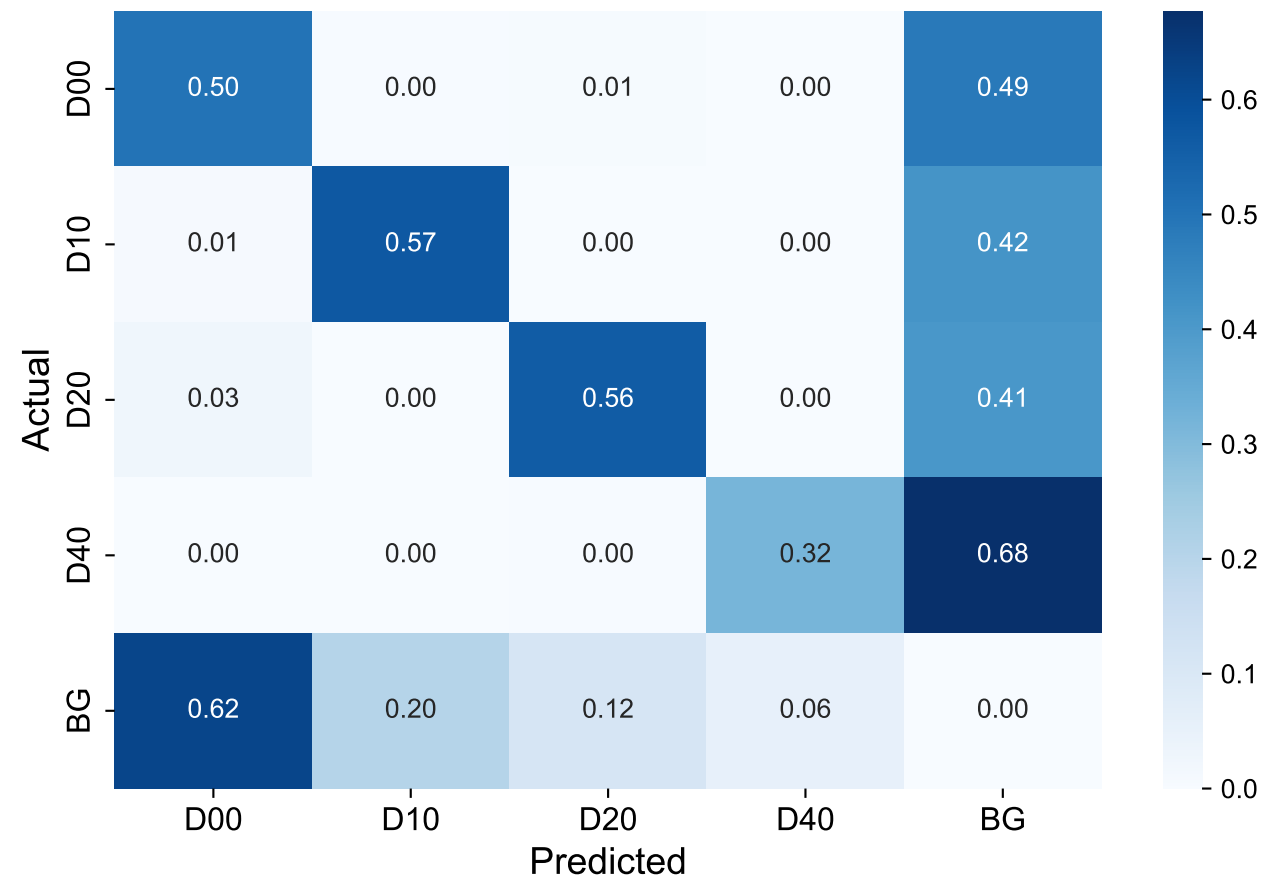
Confusion Matrix for YOLOv8
