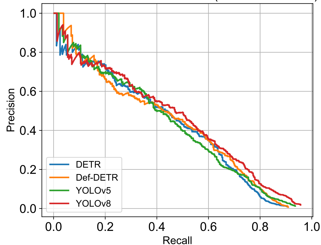
Precision-Recall Curves for D10 (Transverse Crack)
