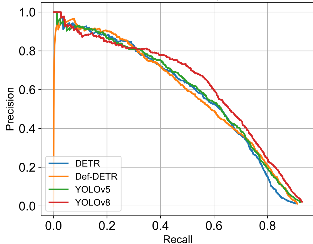
Precision-Recall Curves for D10 (Transverse Crack)
