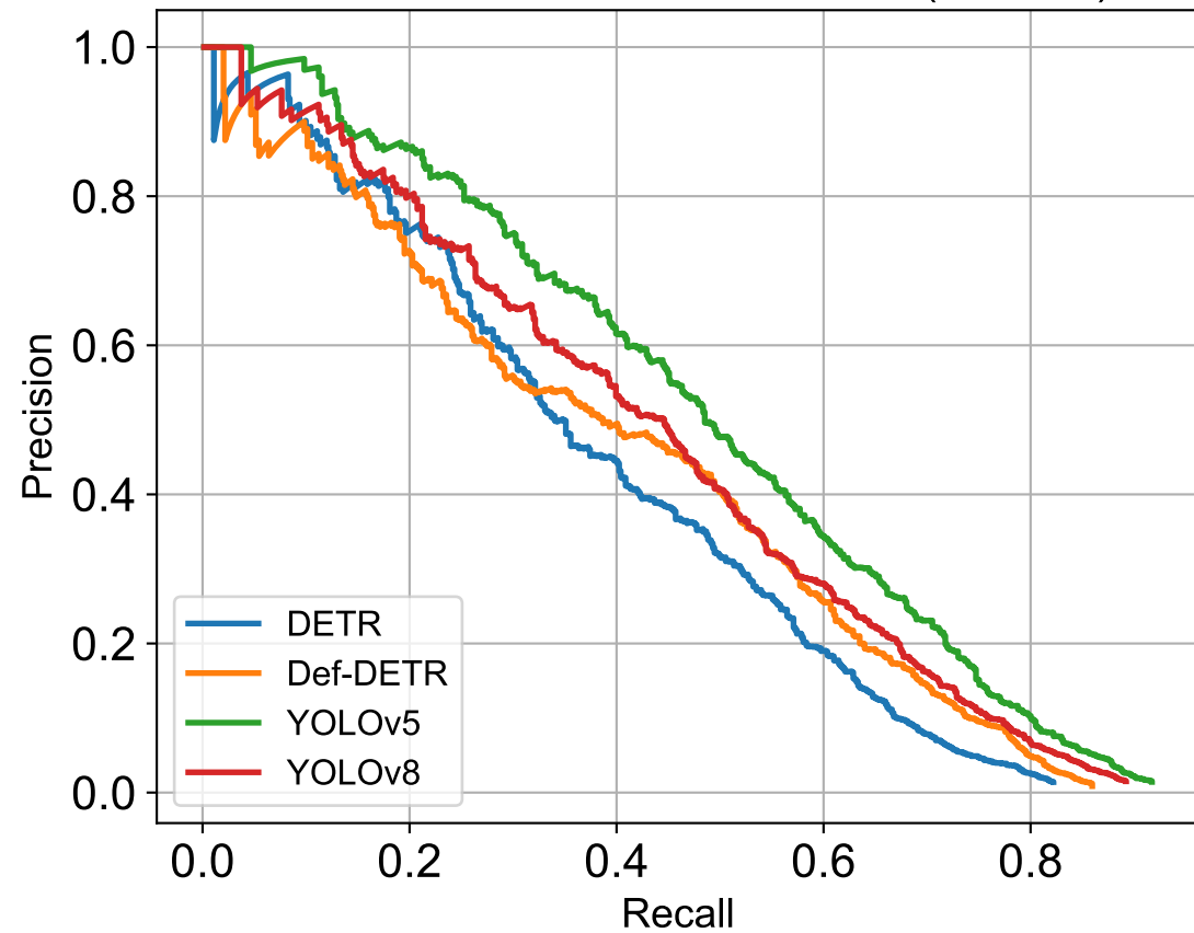
Precision-Recall Curves for D40 (Pothole)
