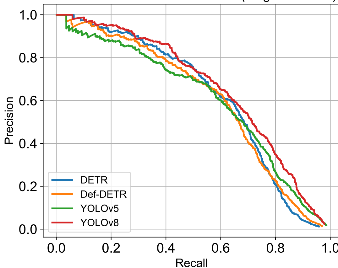
Precision-Recall Curves for D20 (Alligator Crack)
