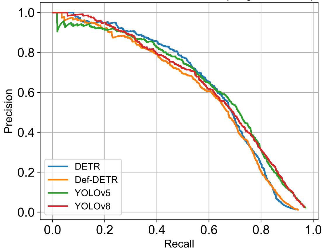
Precision-Recall Curves for D20 (Alligator Crack)
