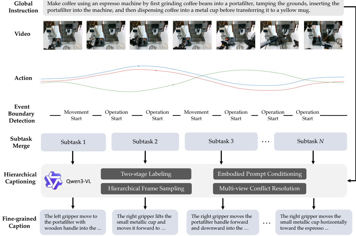
Figure 6: Examples of hierarchical captioning in ManipEvent-5M. The annotation pipeline combines two-stage temporal-semantic labeling, hierarchical episode/event frame sampling, embodied prompt conditioning, and multi-view conflict resolution. The figure shows representative instances that map segmented events to fine-grained captions, complementing the dataset construction pipeline in Fig. 5.
