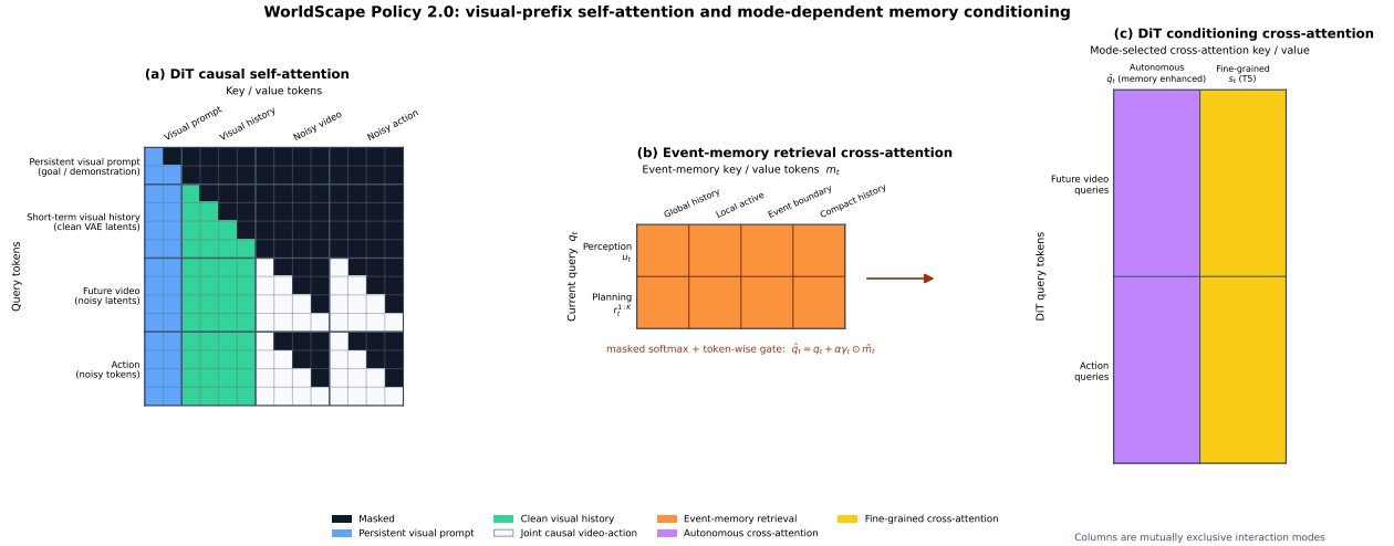
Figure 4: Attention pattern of WorldScape Policy 2.0. In the DiT self-attention mask, persistent visual prompts and clean short-term visual history are placed before the noisy future video and action chunks, so generated tokens can reuse goal, demonstration, and recent observation context without accessing future clean targets. In autonomous planning, event memory is injected through a separate cross-attention path from current reasoning tokens to retrieved global-history, local-active, event-boundary, and compact-history memory tokens; the resulting memory-enhanced VLM tokens condition the DiT. Fine-grained instruction following instead uses T5 tokens as the DiT cross-attention condition.
