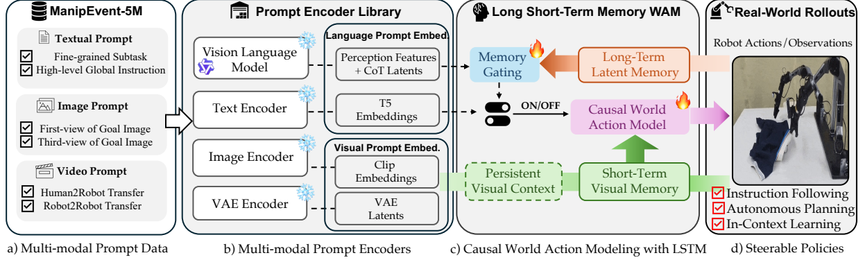
Figure 2: Overview of the WorldScape Policy 2.0 framework. Built on the event-based ManiEvent-5M pretraining data, WorldScape Policy 2.0 encodes observations together with interchangeable text, goal-image, and video-demonstration prompts into a unified causal video-action modeling pipeline. The model couples short-term visual transitions with long-term reasoning-augmented event memory, enabling implicit subgoal planning and joint video-action prediction. This design supports both autonomous planning from coarse task instructions and controllable manipulation from fine-grained subtask captions or visual prompts.
