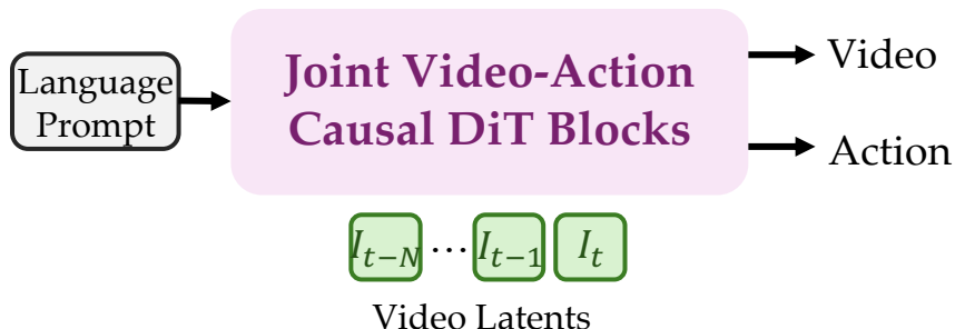
(b) Sliding-Window Memory
