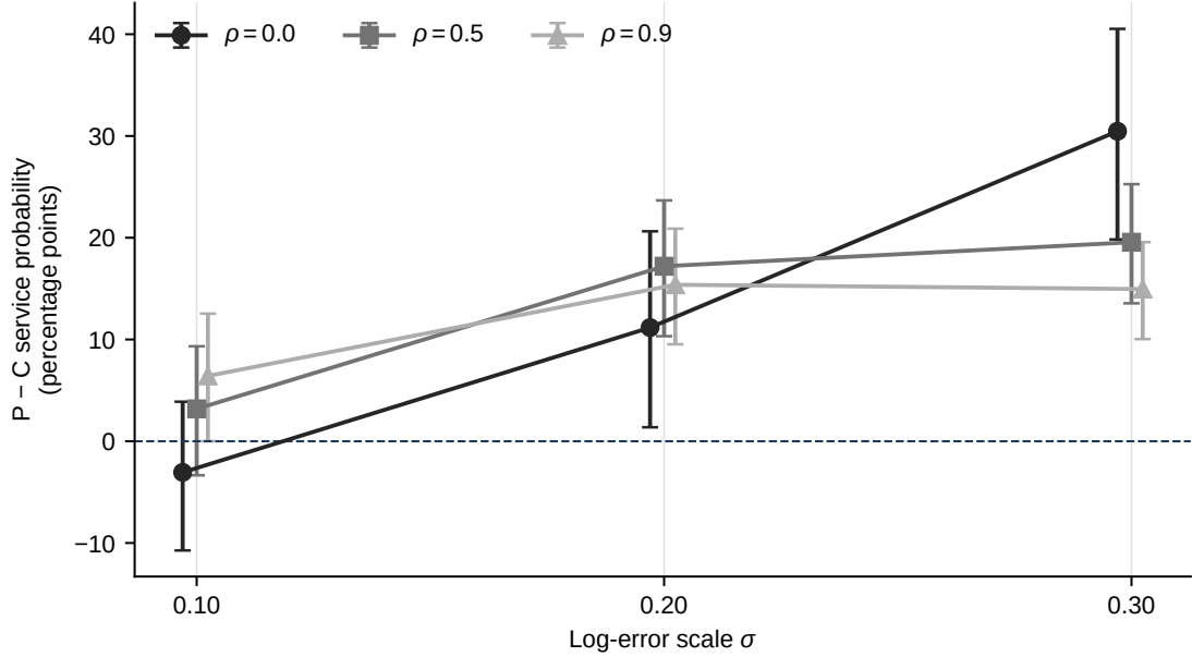
Fig. 1 Paired difference in service probability between the original procedure (P) and conservative-speed planning (C) on the 46 common instances. Circles, squares and triangles mark \rho = 0, 0.5 and 0.9 , and the dashed line marks zero. Faint vertical lines mark \sigma = 0.10, 0.20 and 0.30 ; markers are offset slightly around them only for legibility. Error bars are 95% bootstrap intervals over instances. Plans are fixed across this disturbance sweep, and the intervals are not simultaneous across cells.
