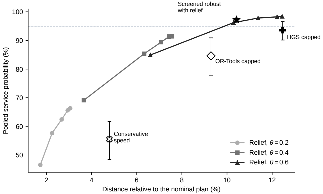
Fig. 2 Pooled validated service-event probability against mean distance relative to the nominal plan of the robust search, on the 45 development instances. Lines join the relieved robust settings for each \theta , from \Gamma = 1 to box uncertainty. The screened procedures (OR-Tools, HGS), screened robust with relief and conservative speed are shown separately, with 95% bootstrap intervals over instances for their service probability. The dashed line marks the 95% target.
