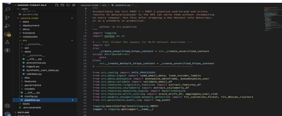
The orchestration layer (src/pipeline.py) that wires each pipeline stage together.
