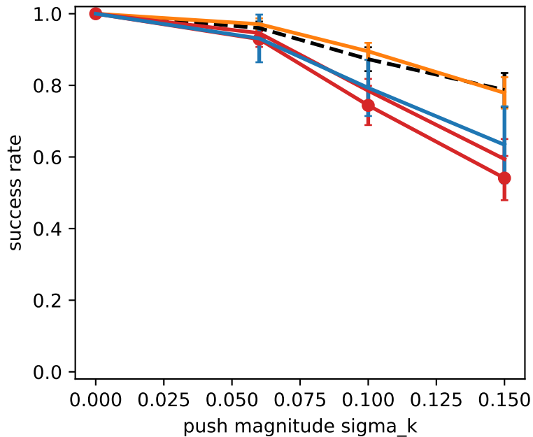
Phase A: point vs cloud, same PD tracker (mean \pm 95% CI over seeds) mild terrain
