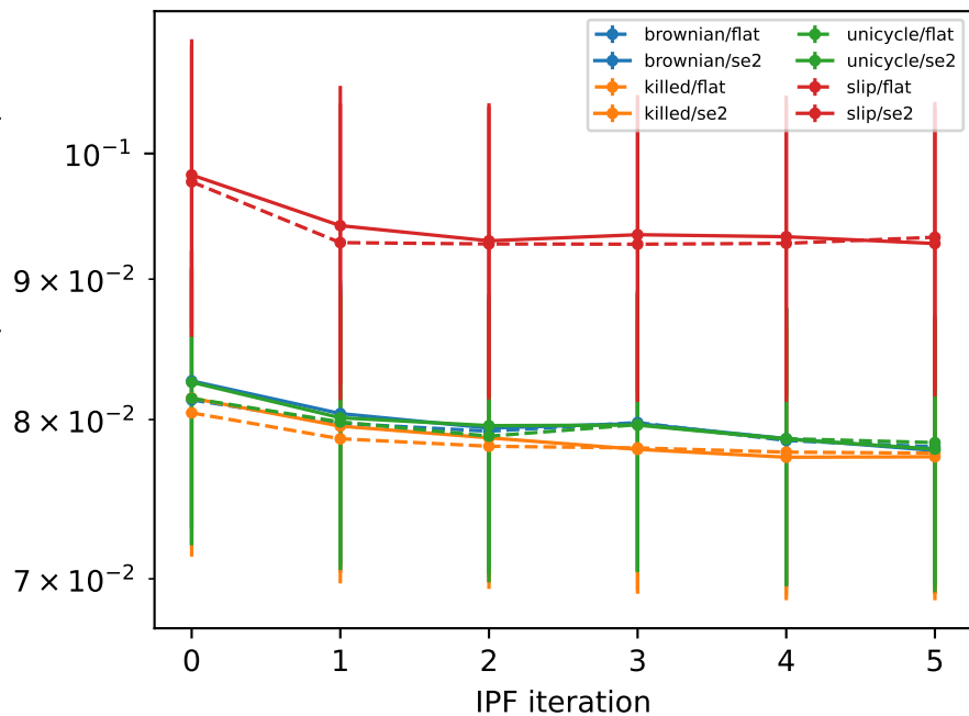
Phase 1: does IPF converge? (pooled over the three skills)
