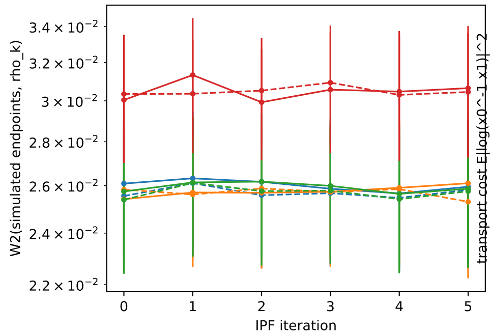
Phase 1: does IPF converge? (pooled over the three skills)
