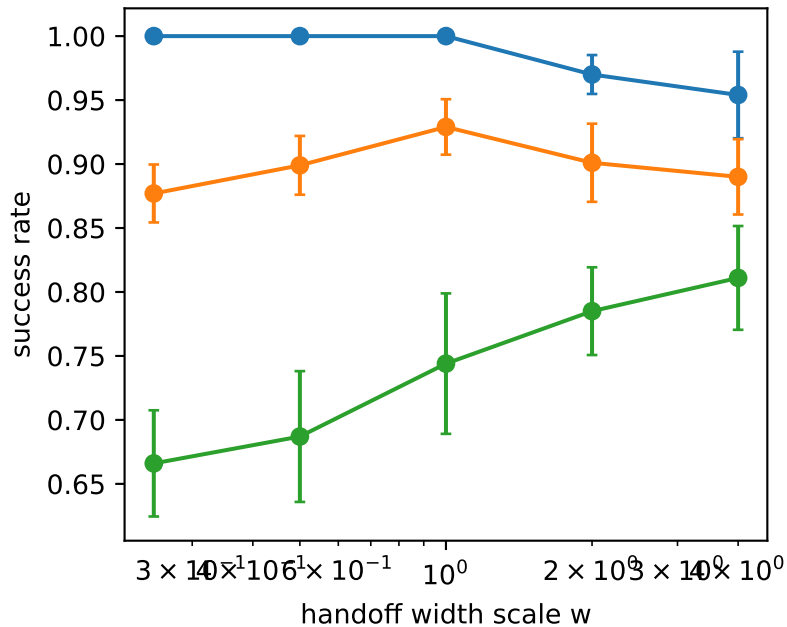
Phase B: handoff-width sweep, BRIDGE-slip-tracked mild terrain
