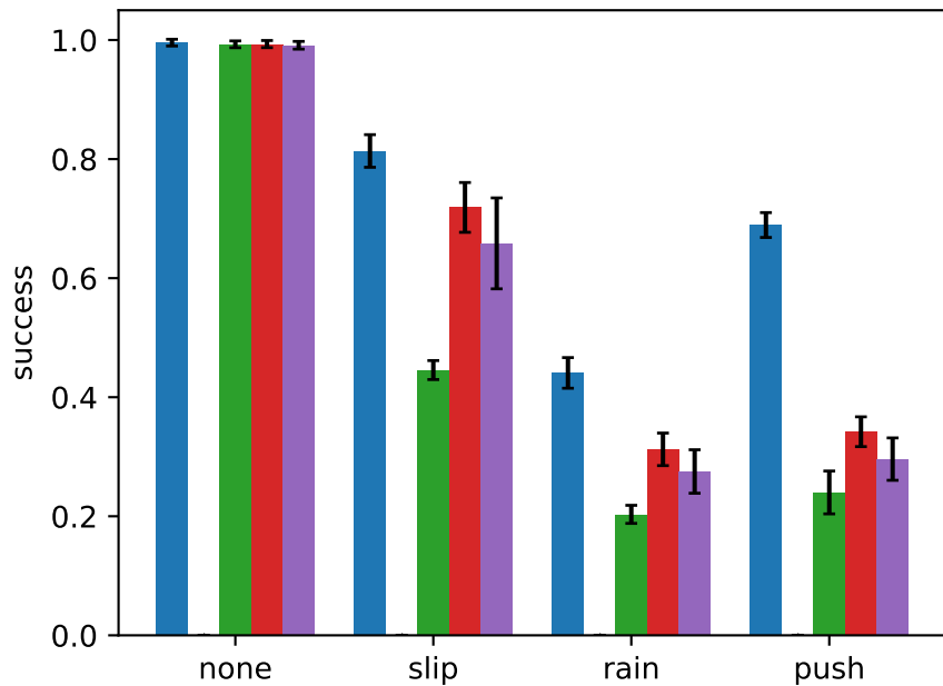
Phase 2: terrain robustness (mean \pm 95% CI over seeds)
