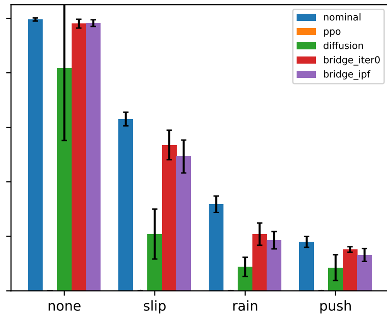
Phase 2: terrain robustness (mean \pm 95% CI over seeds)
