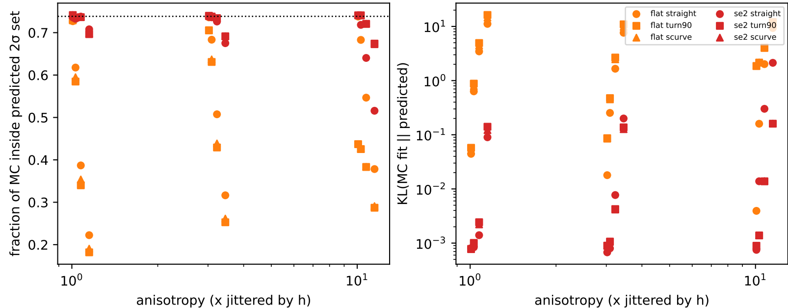
Phase 1b: covariance fidelity, analytic vs 10k Monte-Carlo
