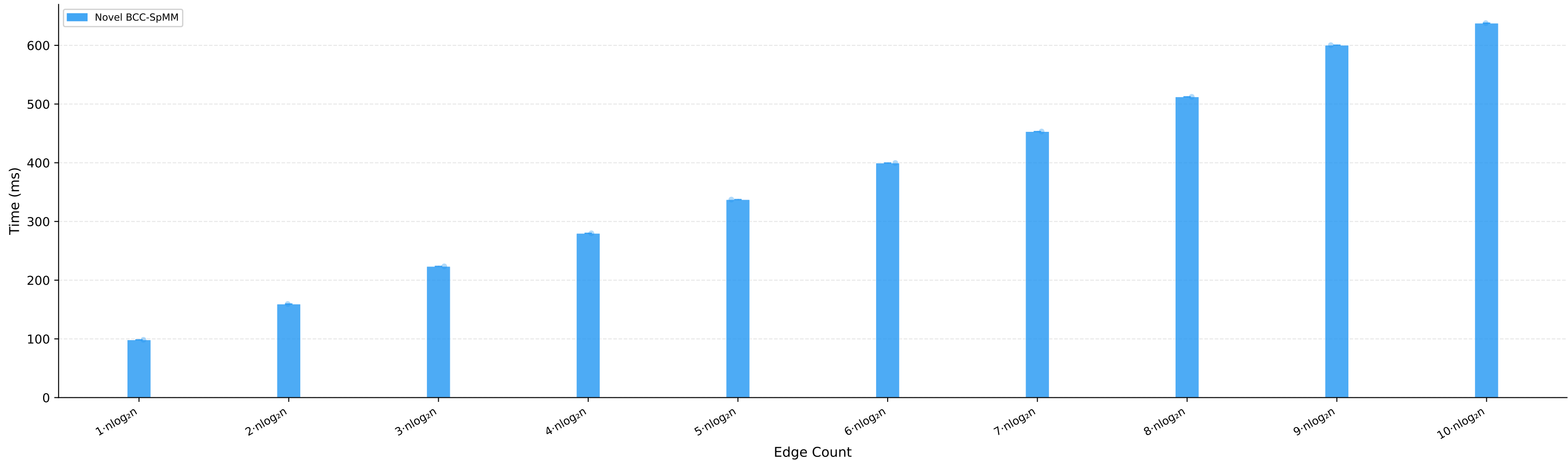
Time vs Number of Edges (n = 50K, threads = 16)
