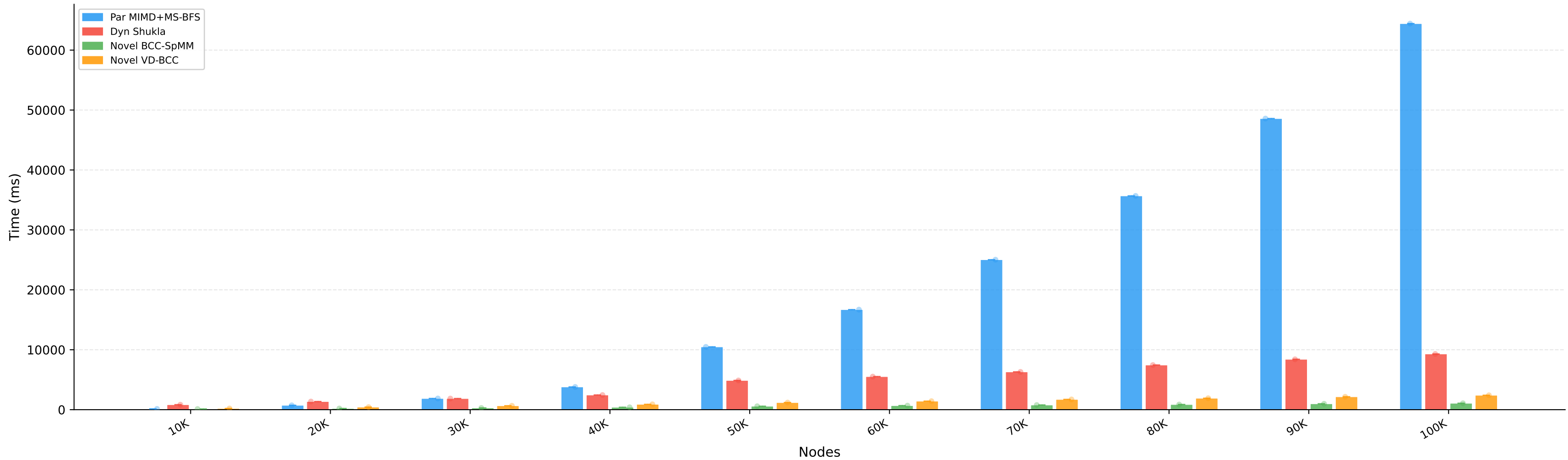
Time vs Number of Nodes (edges = n \cdot \log_2 n , threads = 16)
