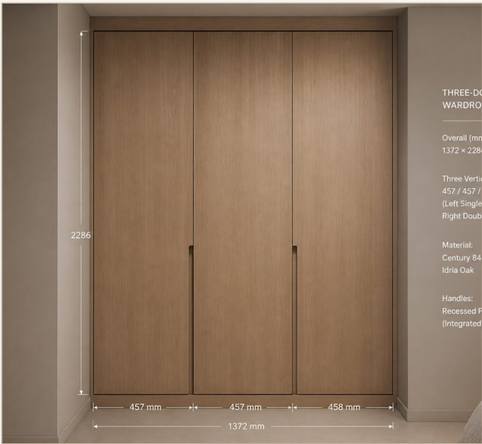
Dimensioned elevation · leaf widths locked to W-01 clear opening
