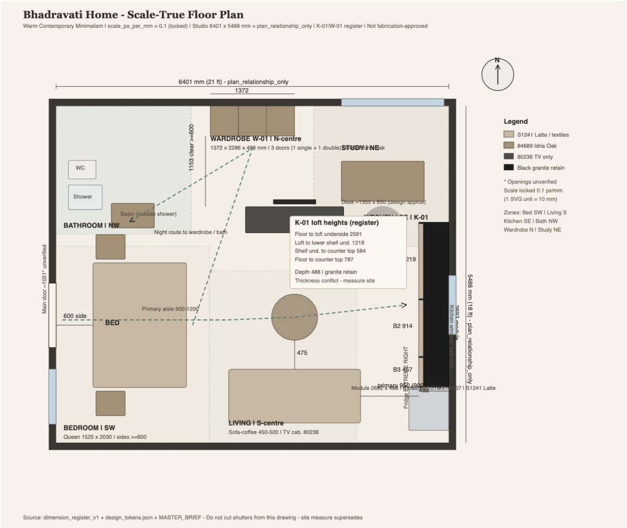
Scale-true plan diagram — relational envelope; fridge extreme right; not a cut sheet
