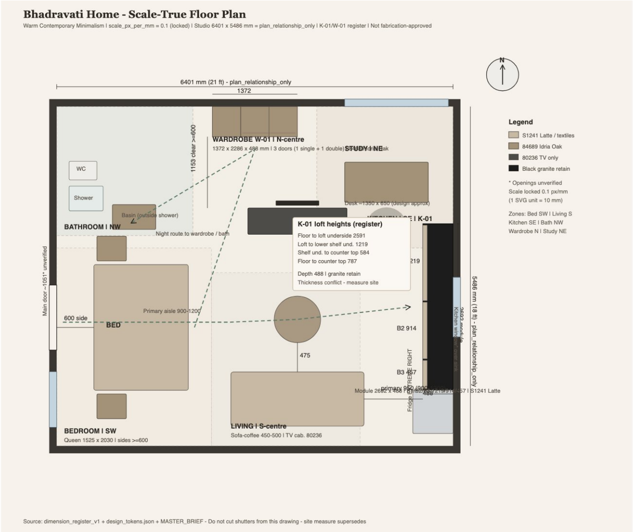
Scale-true dimensioned floor plan (relational; not a cut sheet)
