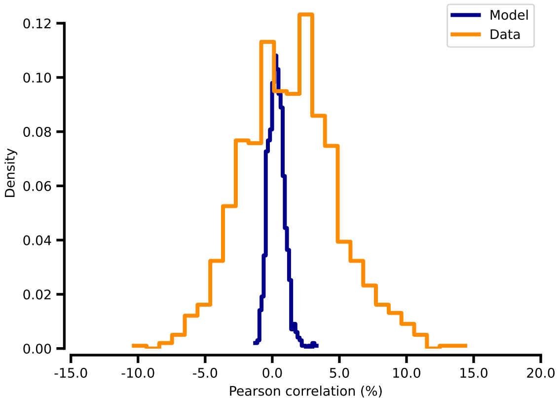
Correlation distributions of x
