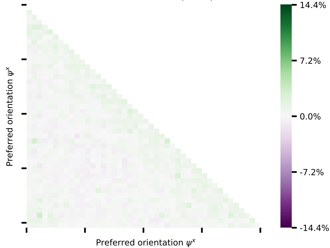
Pearson correlation of x (model)
