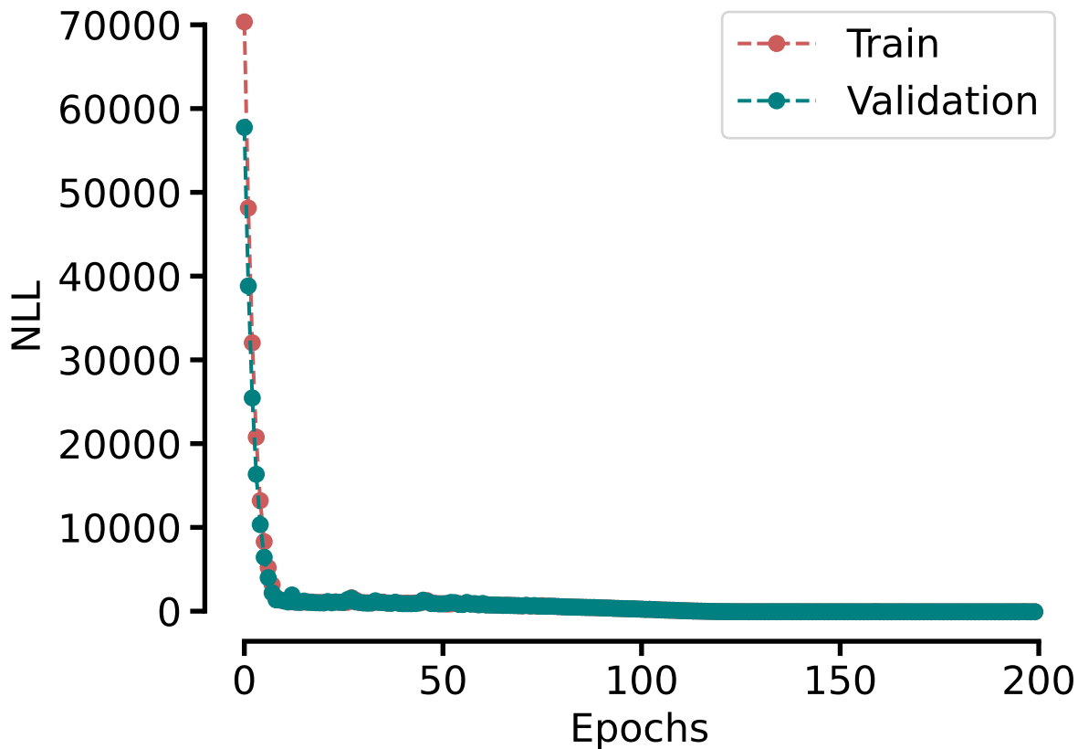
Training and Validation NLL
