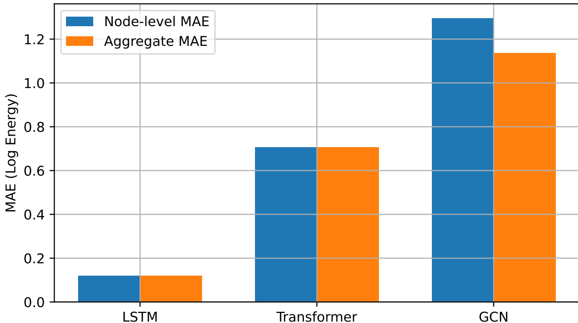
RQ2: Hierarchical GNN vs Temporal Models
