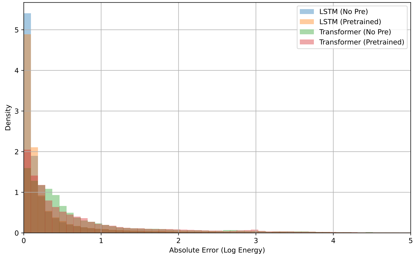
RQ4: Error Distribution under Sensor Failure
