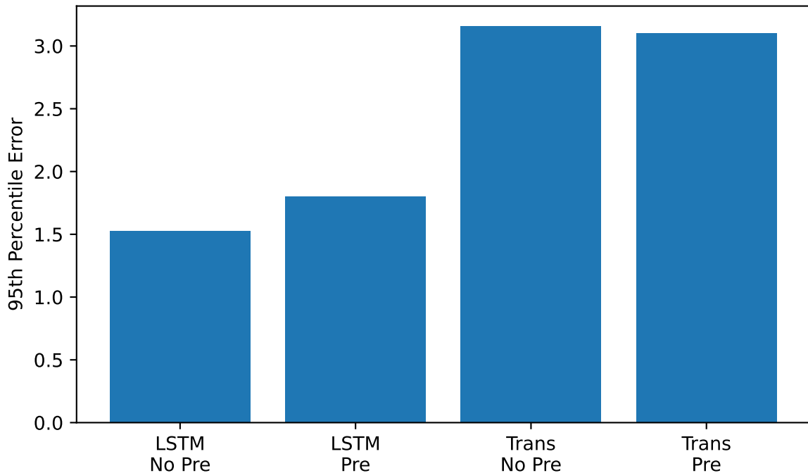
RQ5-F1: Extreme Error Behaviour
