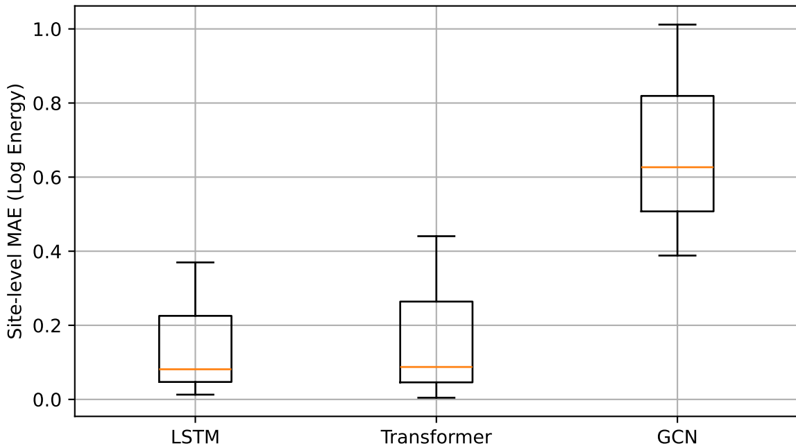
RQ2: Robustness Across Sites (Error Variability)
