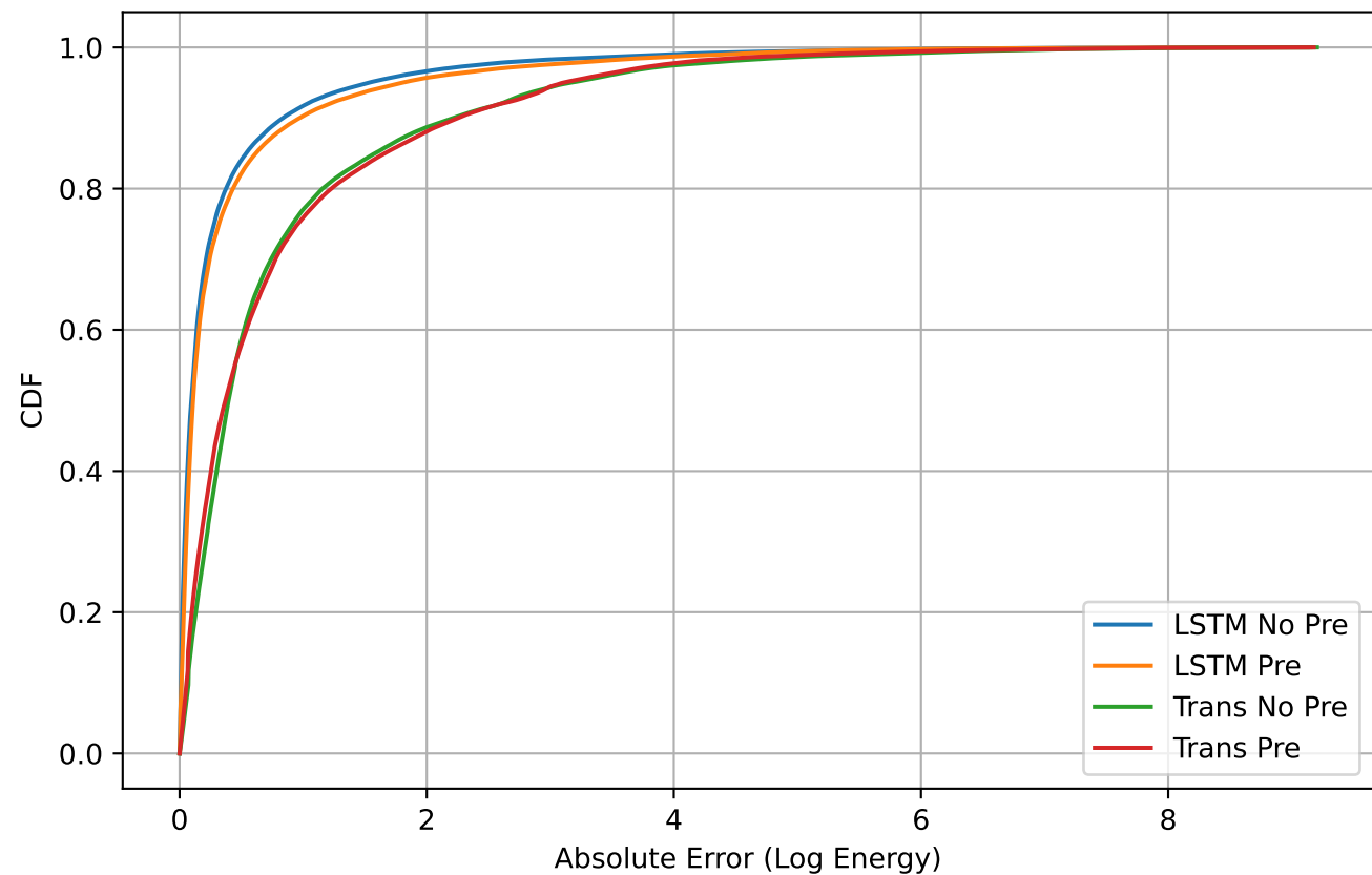
RQ4-F2: Cumulative Error Distribution
