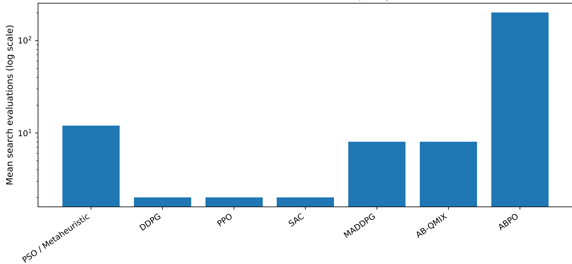
Communication Search Complexity
