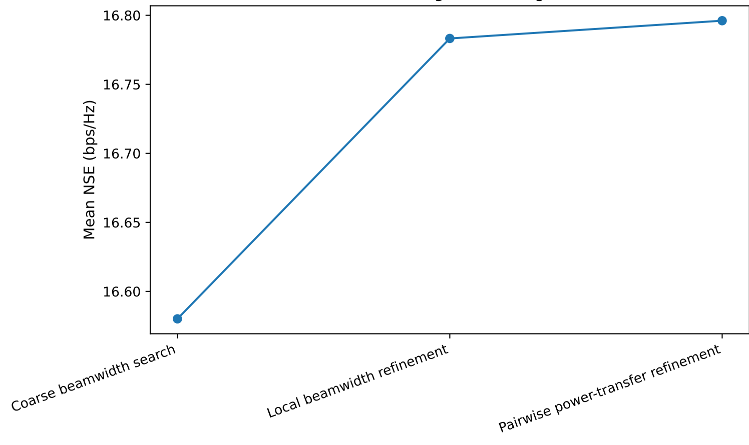
ABPO Search-Stage Score Progression
