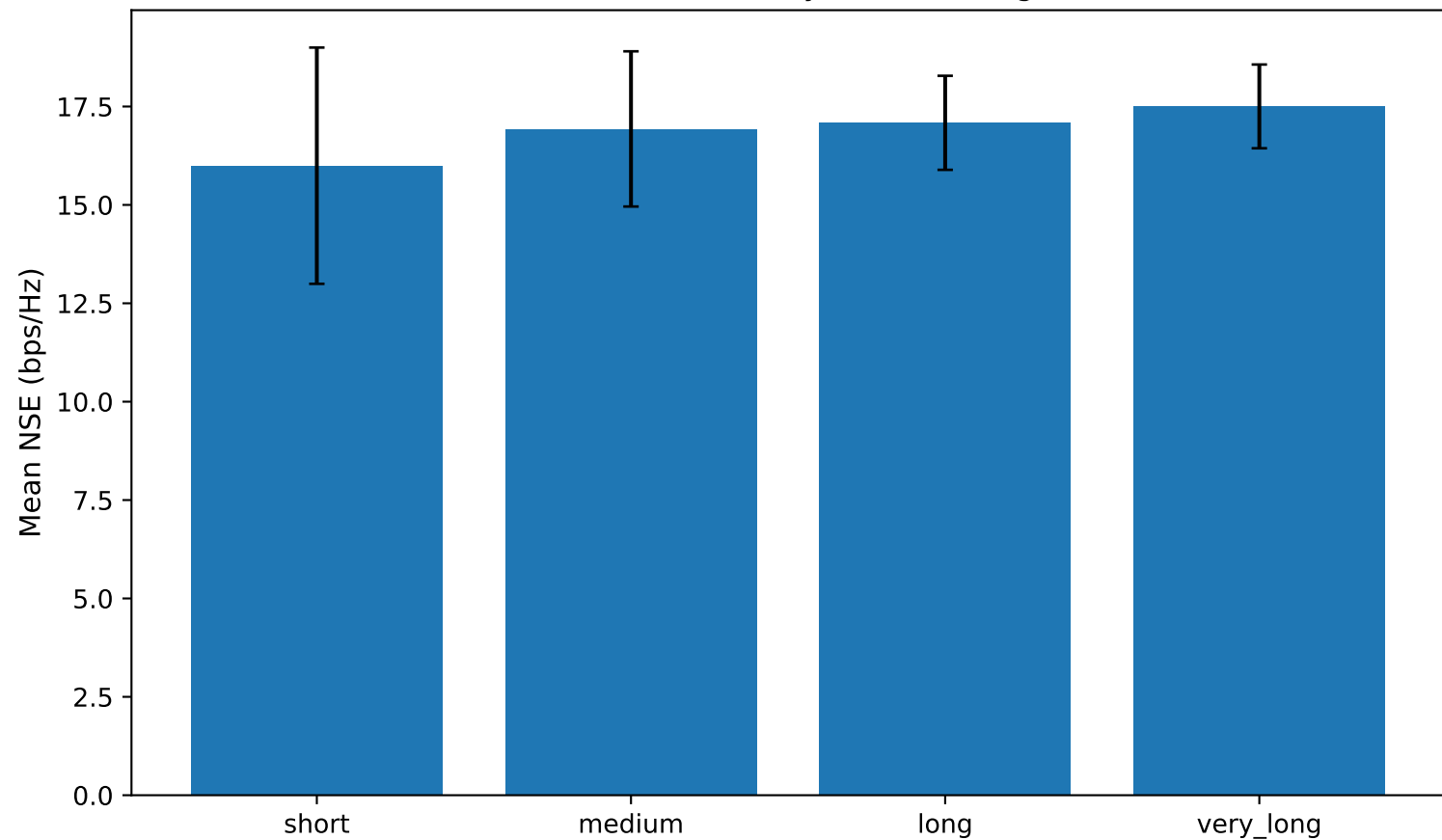
ABPO Performance by Distance Regime
