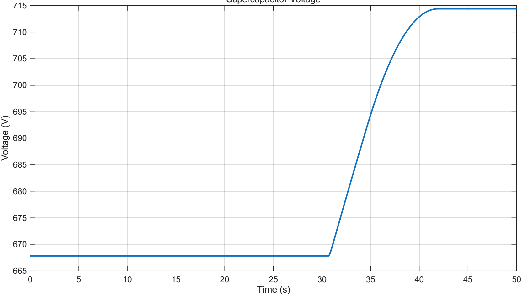
Supercapacitor Voltage
