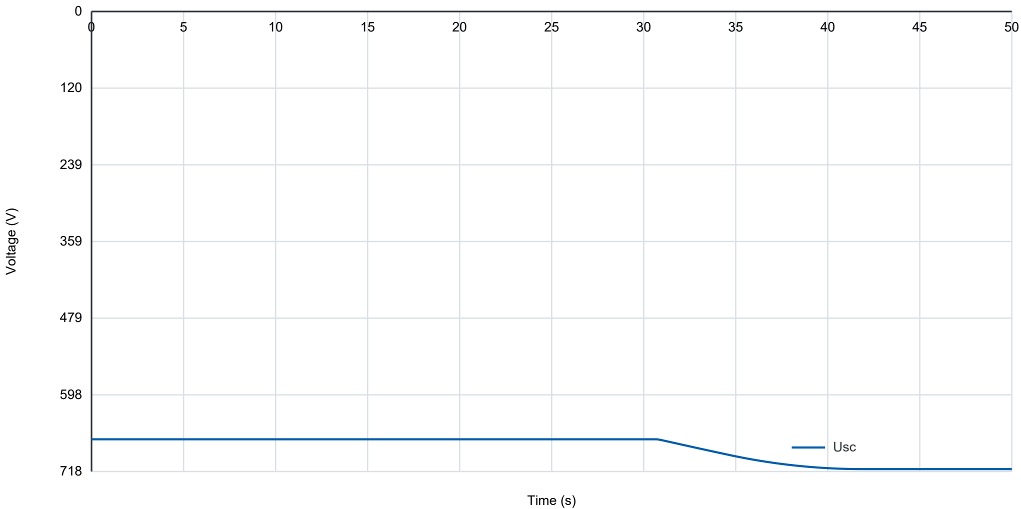
Supercapacitor Voltage vs Time
